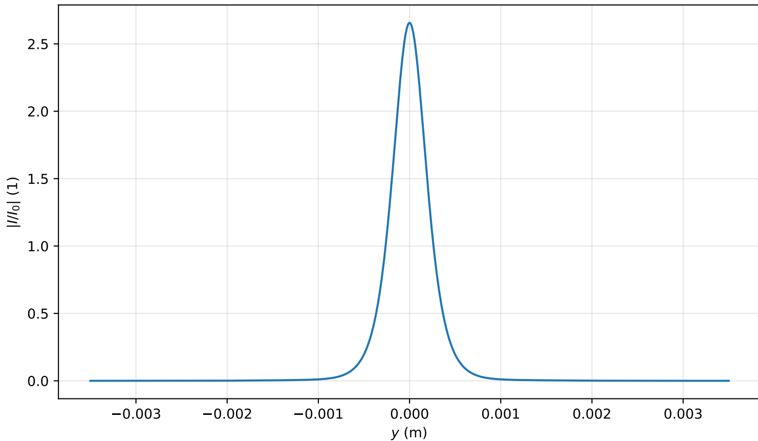
Intensity profile I(x=0, y, z=3.025)/I_0 , \text{Pin}=1.0\text{Pcr} , artificial time
